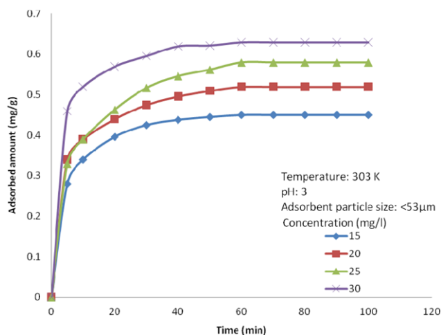
Fig. 2. Effect of time on adsorption amount of Orange G by hematite for different concentrations.
